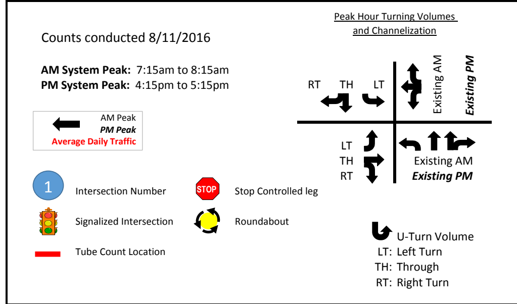
Figure 1: Liberty Lake Network Analysis Intersection Channelization and Volumes: Existing (2016) AM/PM Peak Hours
